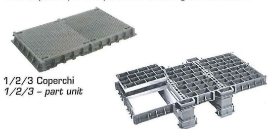
Multiplo a putrelle Multiple unit with removable beams
